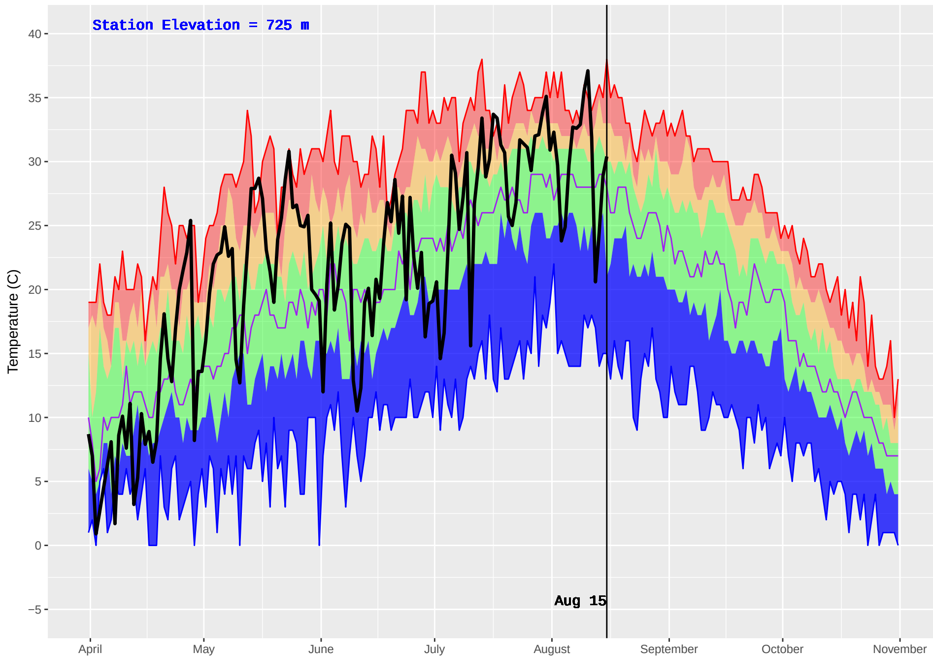
PENDOREILLE (402) : Historical (1986–2016) and Current (2018) Daily Temperature
